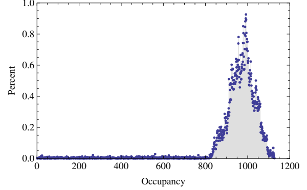
Fig. 6. True queue occupancy in M/M/1 micro-benchmark with software-to-hardware virtual queue.
